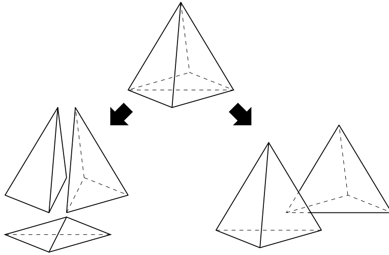
Figure 2.18: This hexahedron can be tetrahedralized in two ways. The Delaunay tetrahedralization (left) includes an arbitrarily thin tetrahedron known as a sliver , which could compromise the accuracy of a finite element simulation. The non-Delaunay tetrahedralization on the right consists of two nicely shaped elements.
