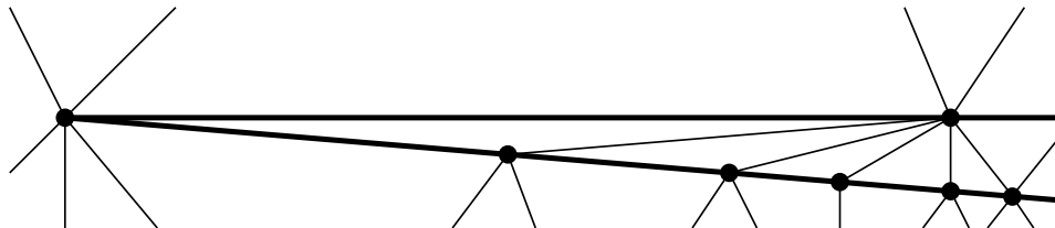
Figure 3.36: The simplest method of ensuring termination when small input angles are present has undesirable properties, including the production of large angles and many small angles.
