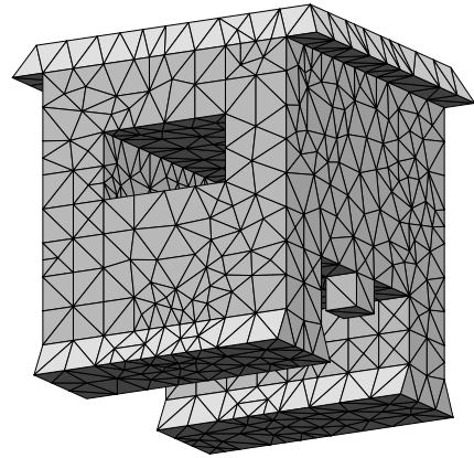
Figure 4.22: Meshes created by Delaunay refinement with bounds on the smallest dihedral angle \theta_{\min} . Also listed for each mesh is its largest dihedral angle \theta_{\max} and its shortest edge length h_{\min} . Compare with Figure 4.18 on Page 105.
