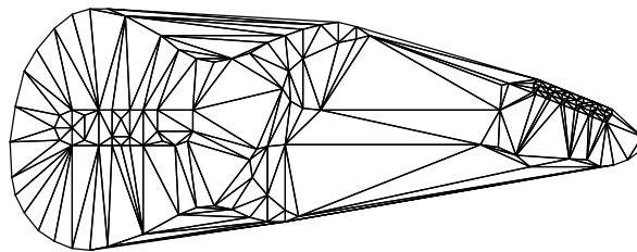
Figure 3.20: Constrained Delaunay triangulation of PSLG.
