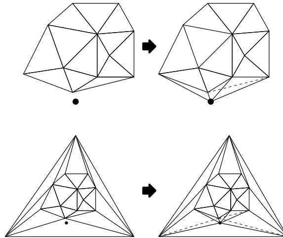
Figure 2.36: Top: A vertex is inserted outside the convex hull of the previously existing vertices. Bottom: A triangular bounding box is used so that all vertex insertions are internal. In practice, the bounding box should be much larger than the one depicted here. Even then, problems may arise.
