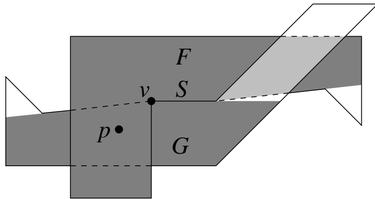
Figure 4.15: Two incident facets separated by a dihedral angle of nearly 180^\circ . The definition of local feature size should not approach zero near v , but it is nonetheless difficult to mesh the region between F and G near v .
