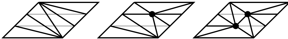
Figure 3.10: In this example, two segments (thin lines) must be recovered. The first is successfully recovered with a single vertex insertion, but the attempt to recover the second eliminates a subsegment of the first.
