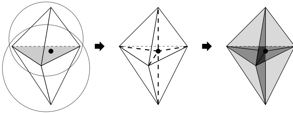
Figure 2.33: The Bowyer/Watson algorithm in three dimensions. At left, a new vertex falls inside the circumcircles of the two tetrahedra illustrated. (These tetrahedra may be surrounded by other tetrahedra, which for clarity are not shown.) These tetrahedra are deleted, along with the face (shaded) between them. At center, the five new Delaunay edges (bold dashed lines). At right, the nine new Delaunay faces (one for each edge of the insertion polyhedron) appear translucent. Six new tetrahedra are formed.
