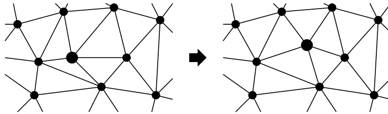
Figure 2.46: Laplacian smoothing.
