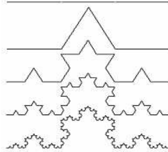
Figure 2.3: Construction of the von Koch curve
