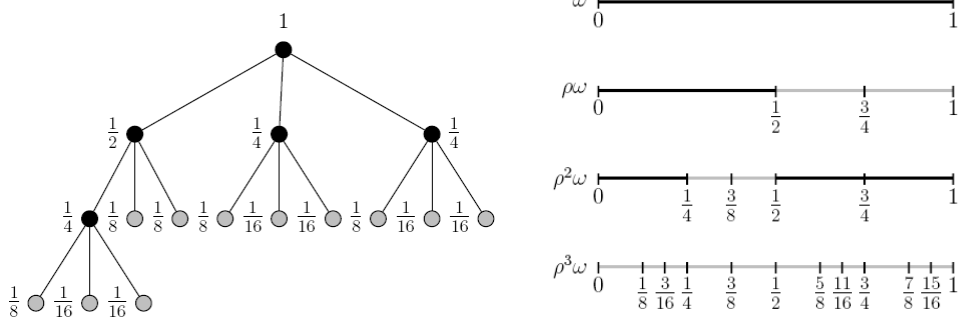
(c) III step
