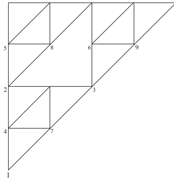
Figure 2.5: Construction of a u.d. sequence of points on T (II step)
