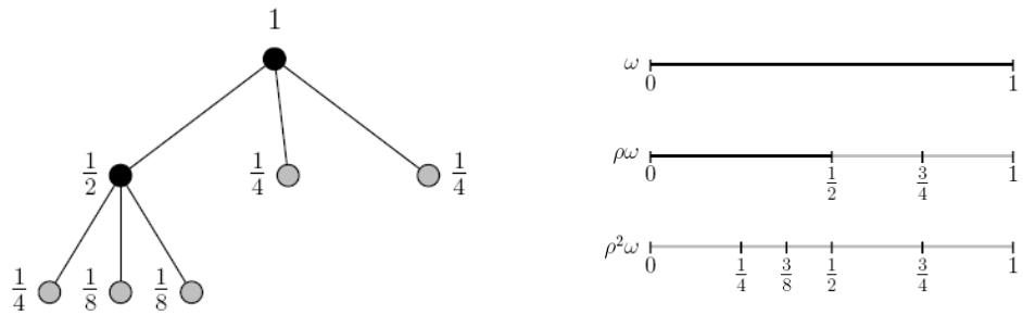
(b) II step
